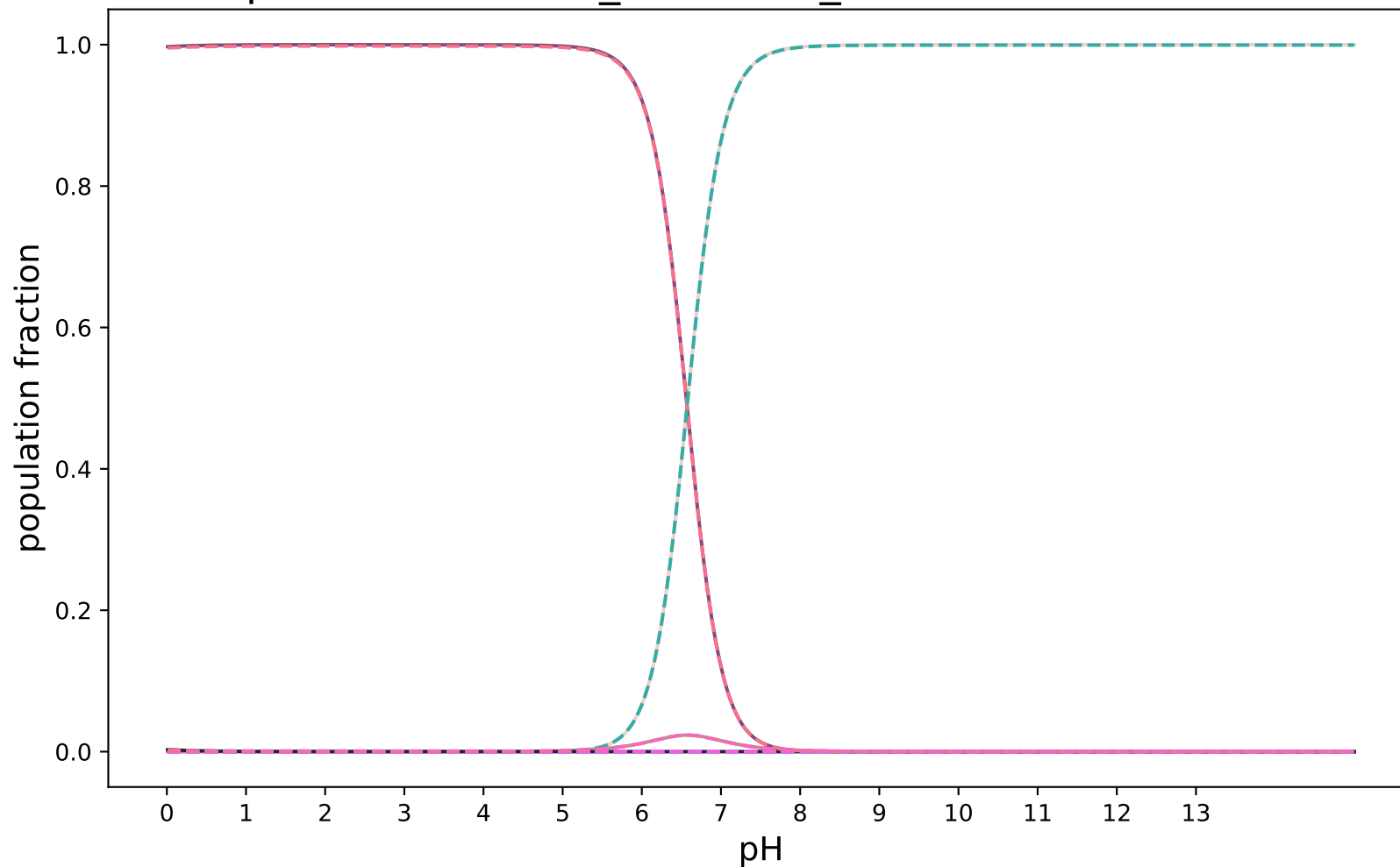
pKa-RobertRaddi_AdaBoost_modified:SAMPL8-19
