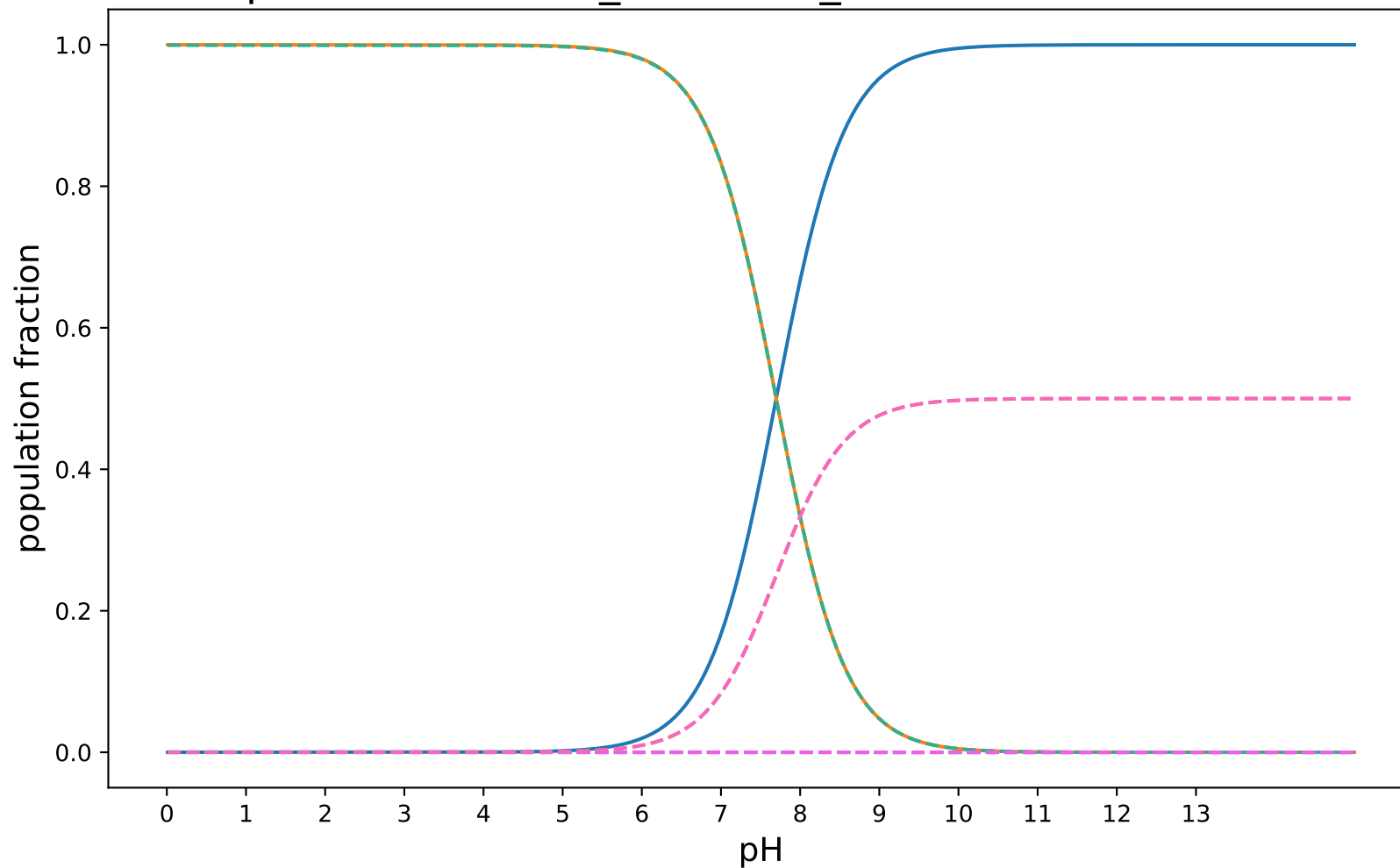
pKa-RobertRaddi_AdaBoost_modified:SAMPL8-20
