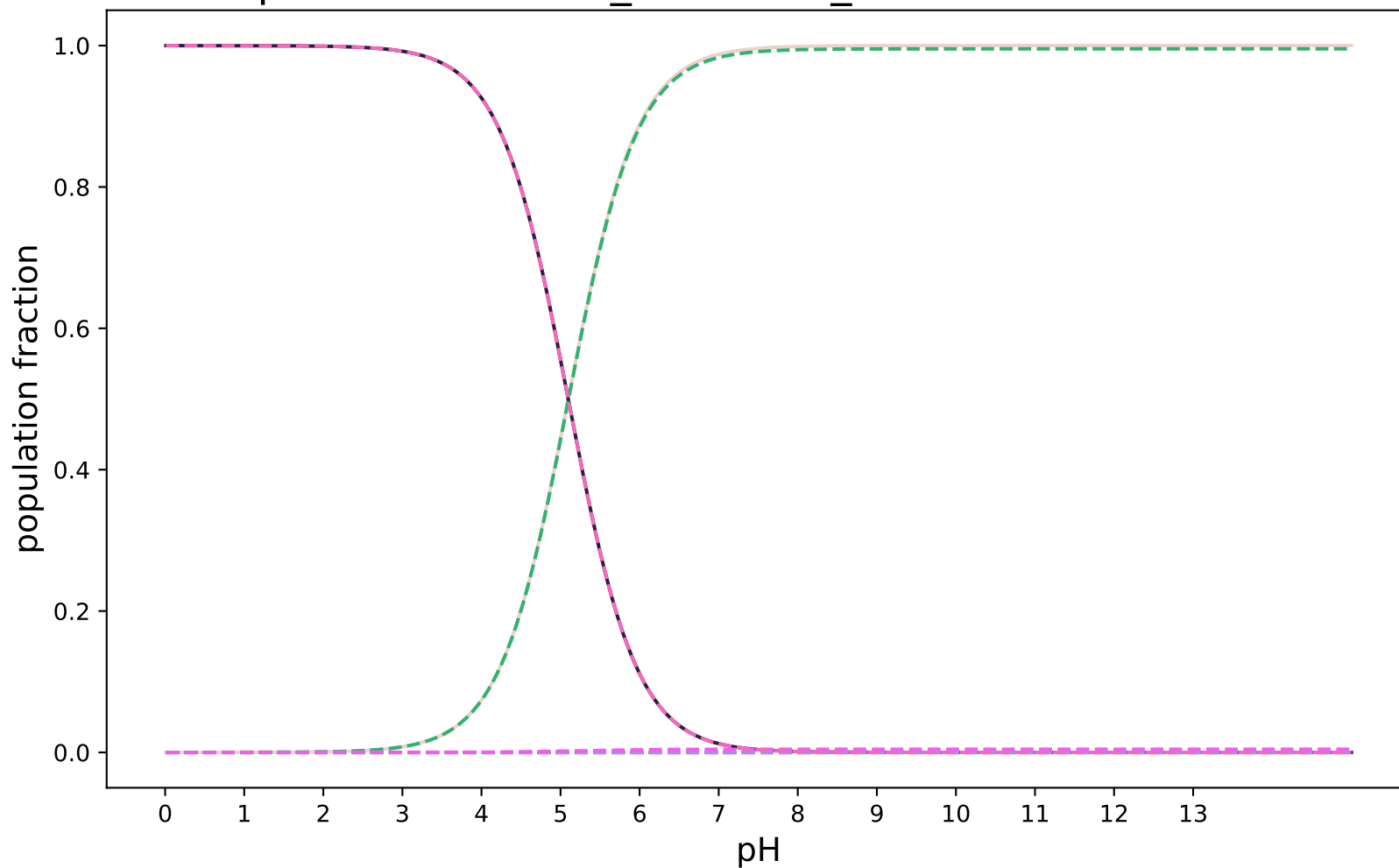
pKa-RobertRaddi_AdaBoost_modified:SAMPL8-3
