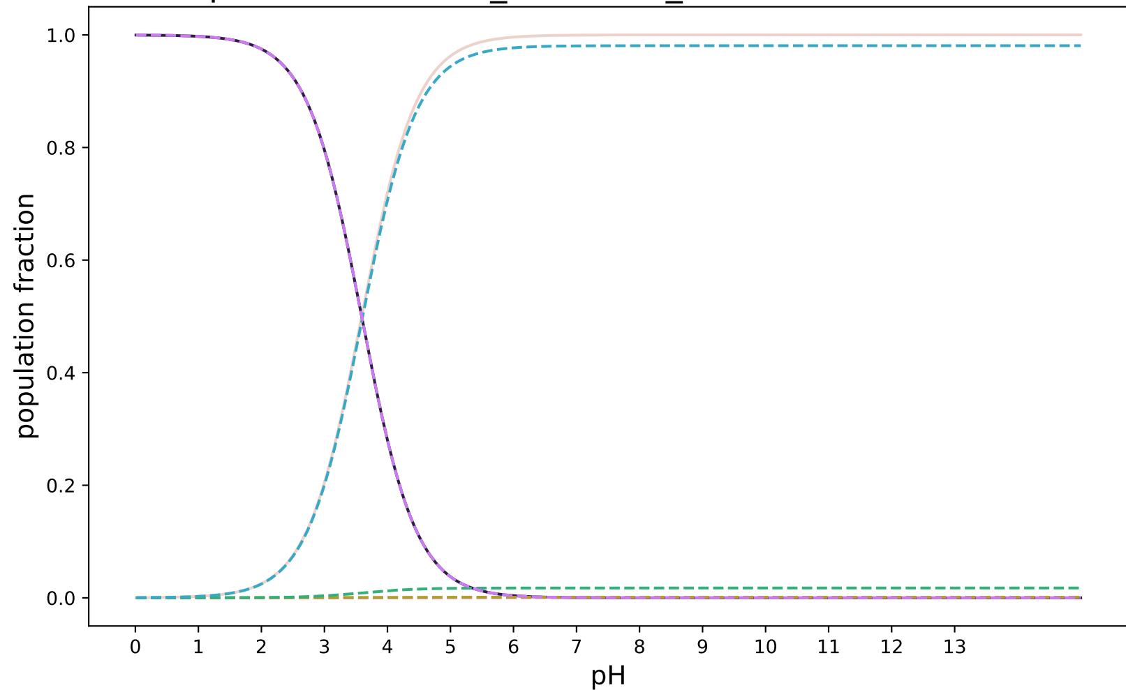
pKa-RobertRaddi_AdaBoost_modified:SAMPL8-4
