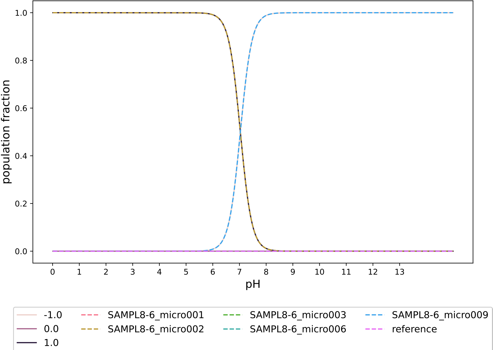
pKa-RobertRaddi AdaBoost modified:SAMPL8-6
