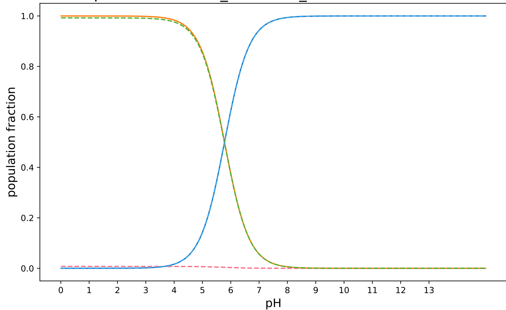
pKa-RobertRaddi_AdaBoost_modified:SAMPL8-8
