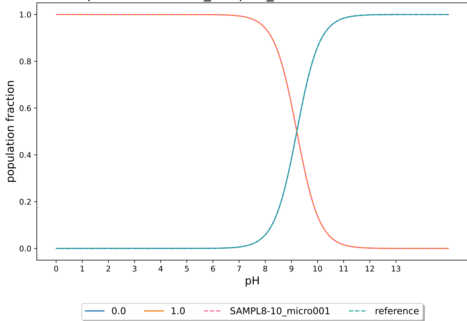
pKa-RobertRaddi_DeepGP_modified:SAMPL8-10
