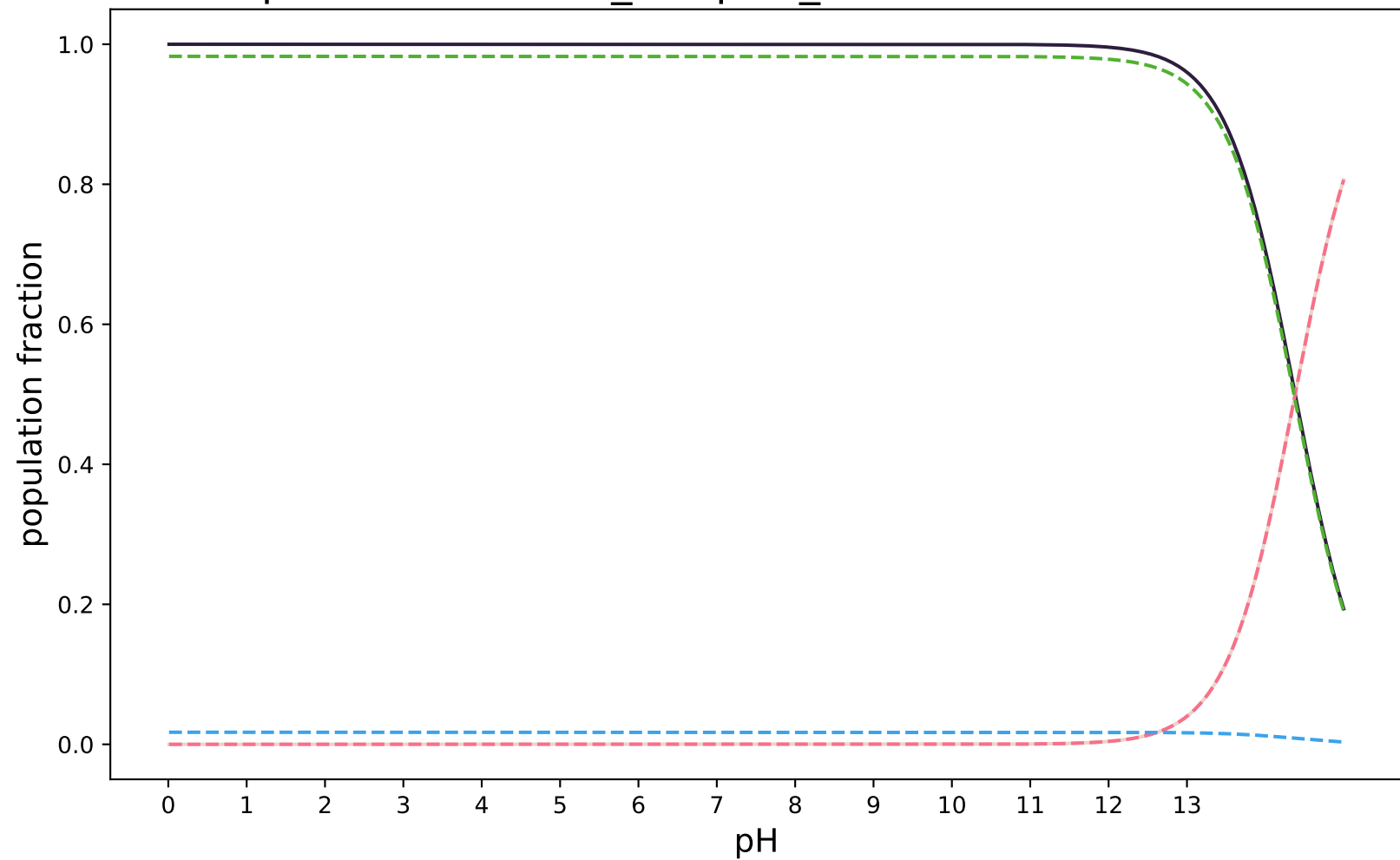
pKa-RobertRaddi_DeepGP_modified:SAMPL8-12
