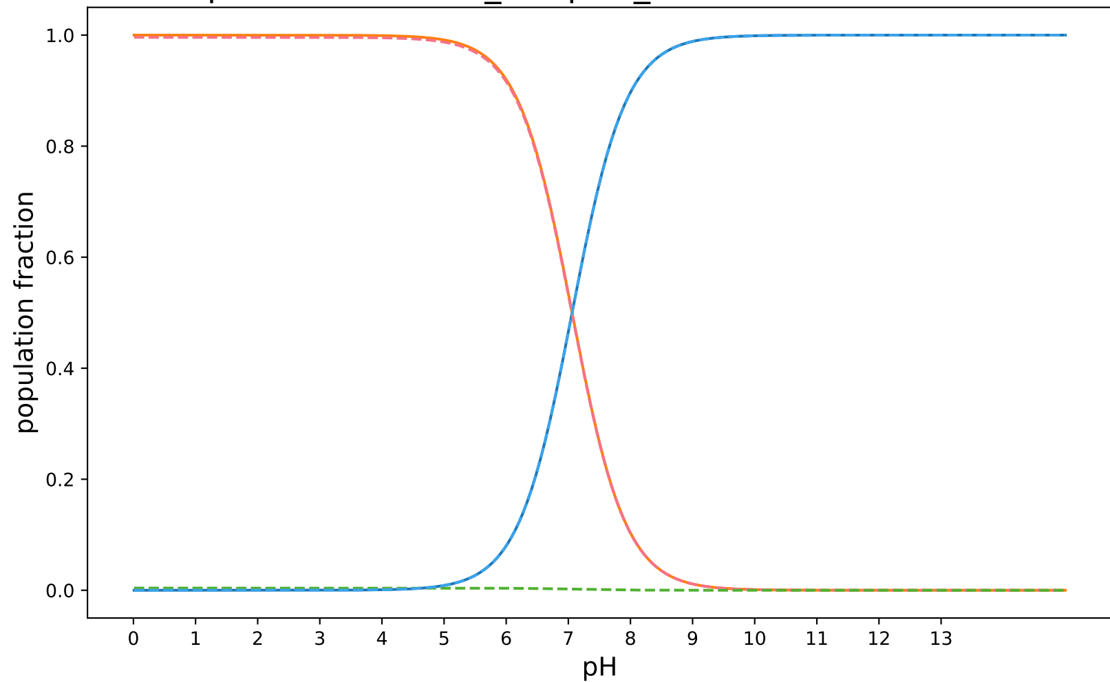
pKa-RobertRaddi_DeepGP_modified:SAMPL8-15
