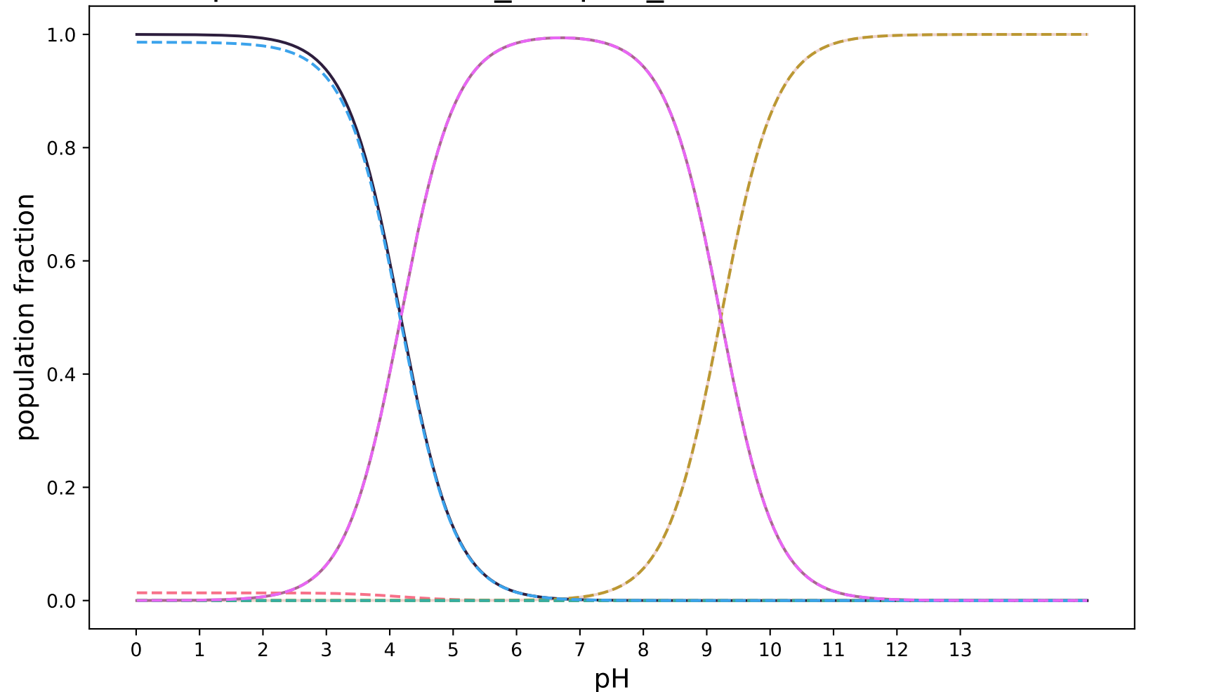
pKa-RobertRaddi_DeepGP_modified:SAMPL8-23
