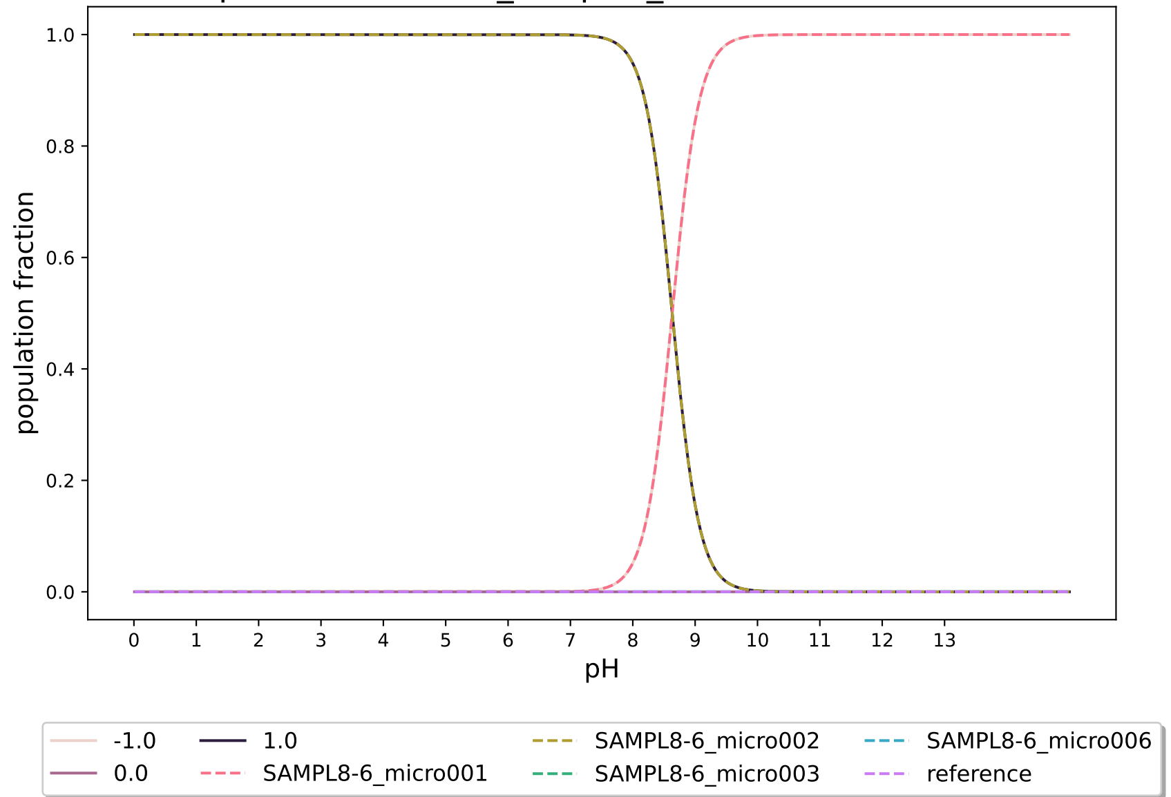
pKa-RobertRaddi_DeepGP_modified:SAMPL8-6
