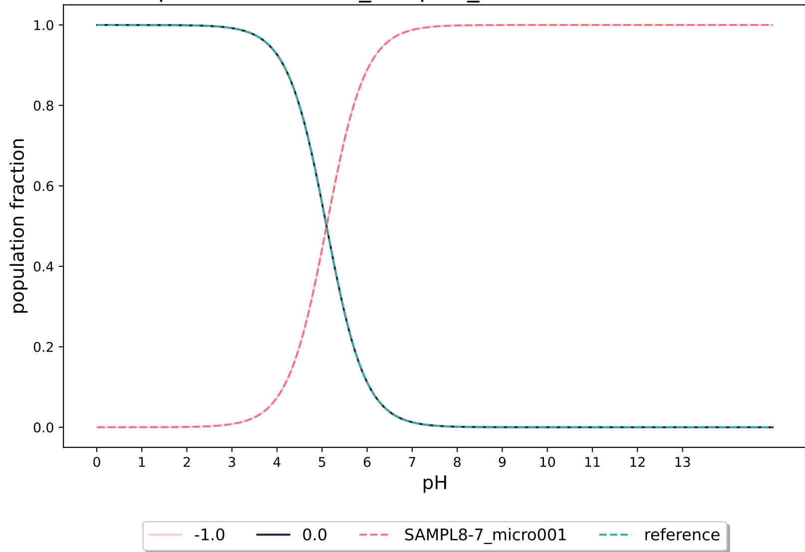
pKa-RobertRaddi_DeepGP_modified:SAMPL8-7
