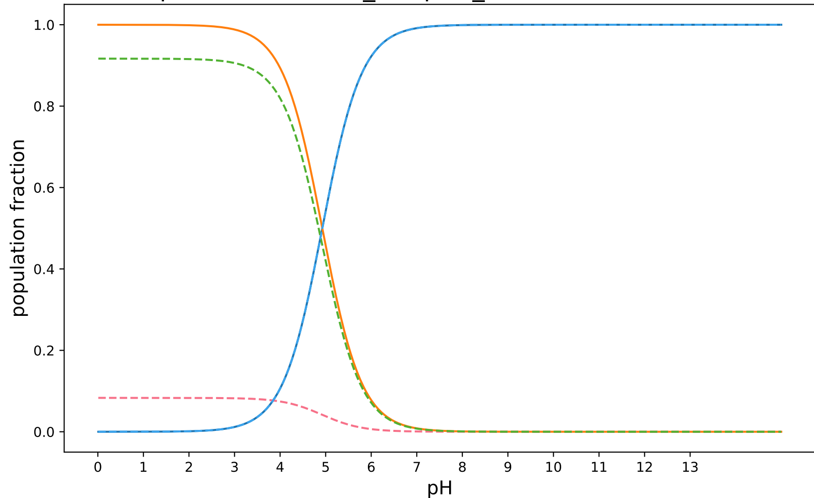
pKa-RobertRaddi_DeepGP_modified:SAMPL8-8
