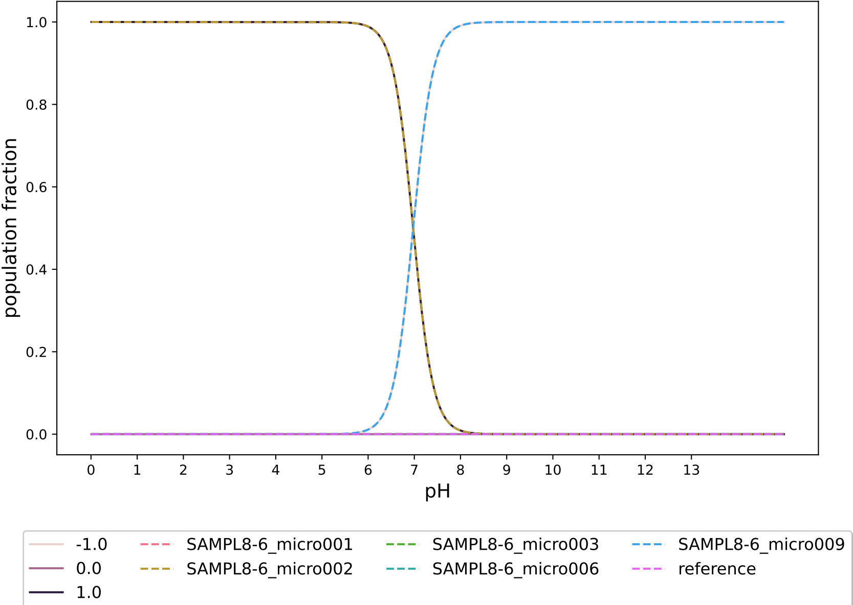
pKa-RobertRaddi RF modified:SAMPL8-6
