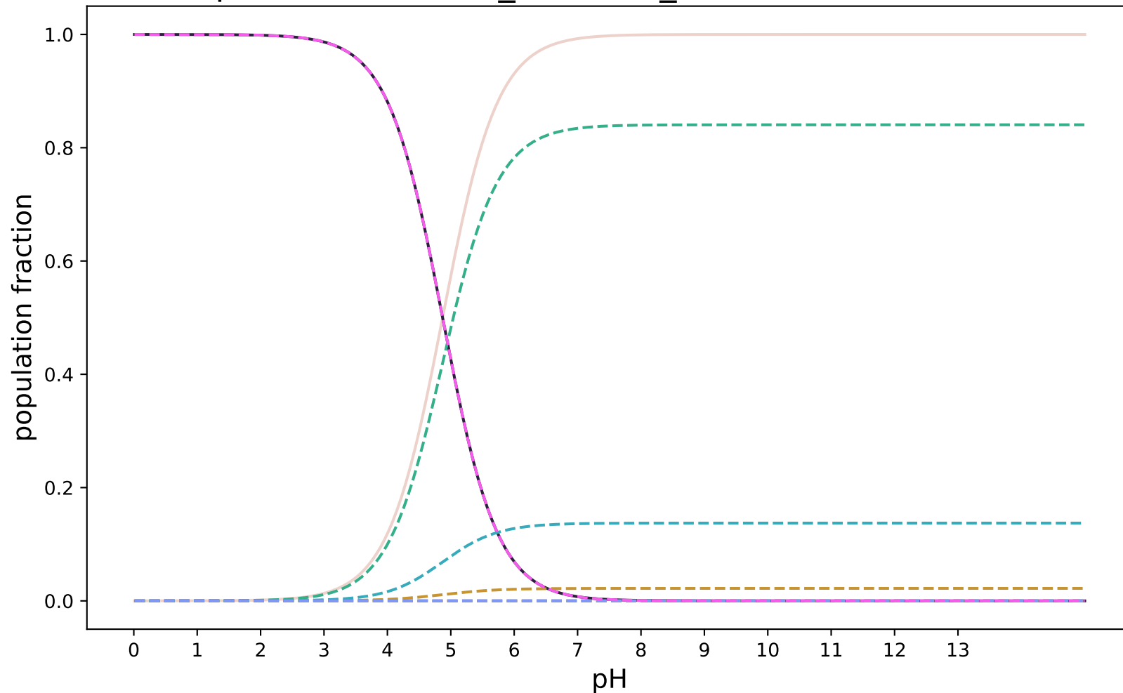
pKa-RobertRaddi_XGBoost_modified:SAMPL8-1
