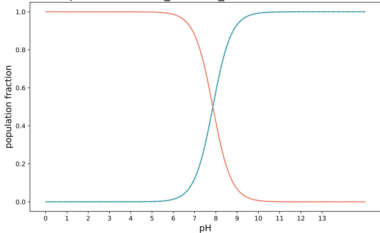
pKa-RobertRaddi_XGBoost_modified:SAMPL8-10
