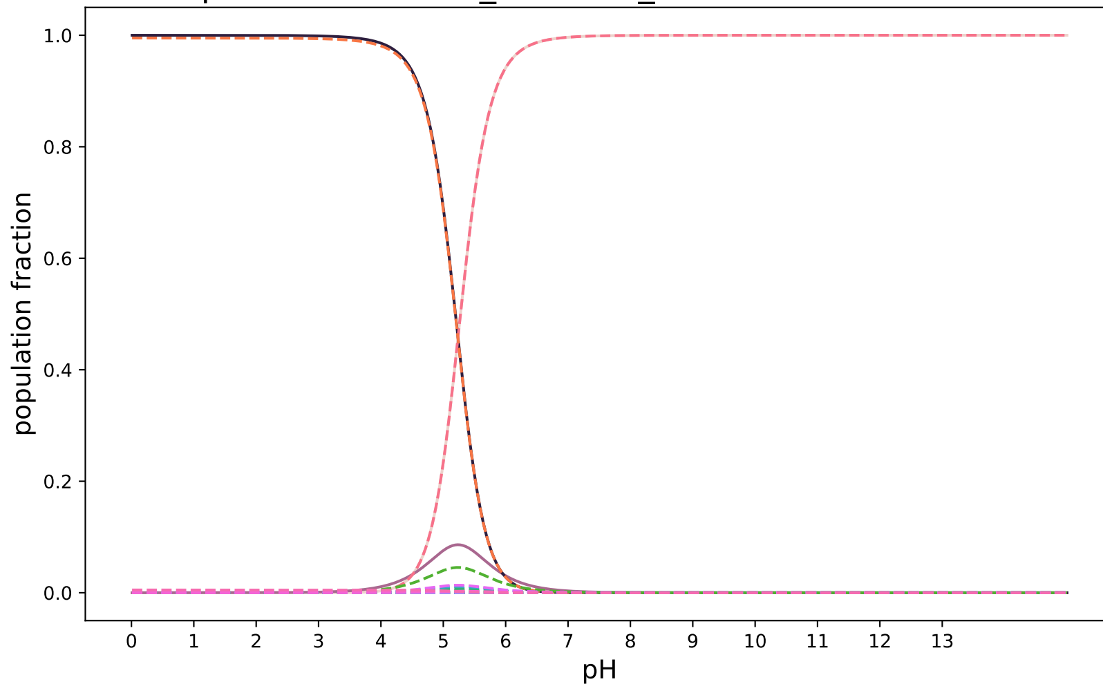
pKa-RobertRaddi_XGBoost_modified:SAMPL8-14
