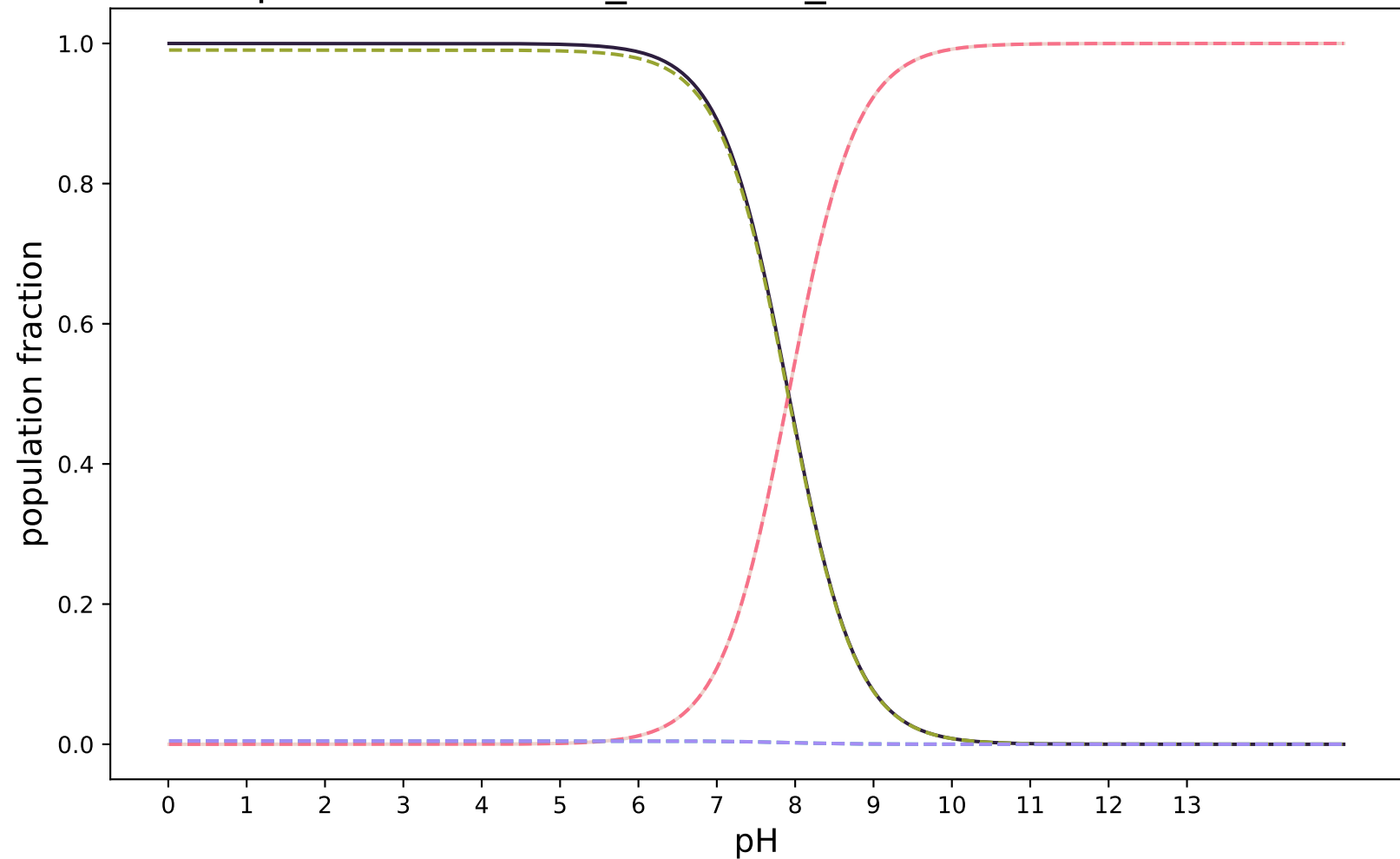
pKa-RobertRaddi_XGBoost_modified:SAMPL8-22
