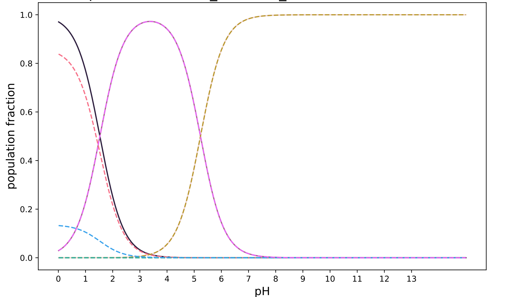
pKa-RobertRaddi_XGBoost_modified:SAMPL8-23
