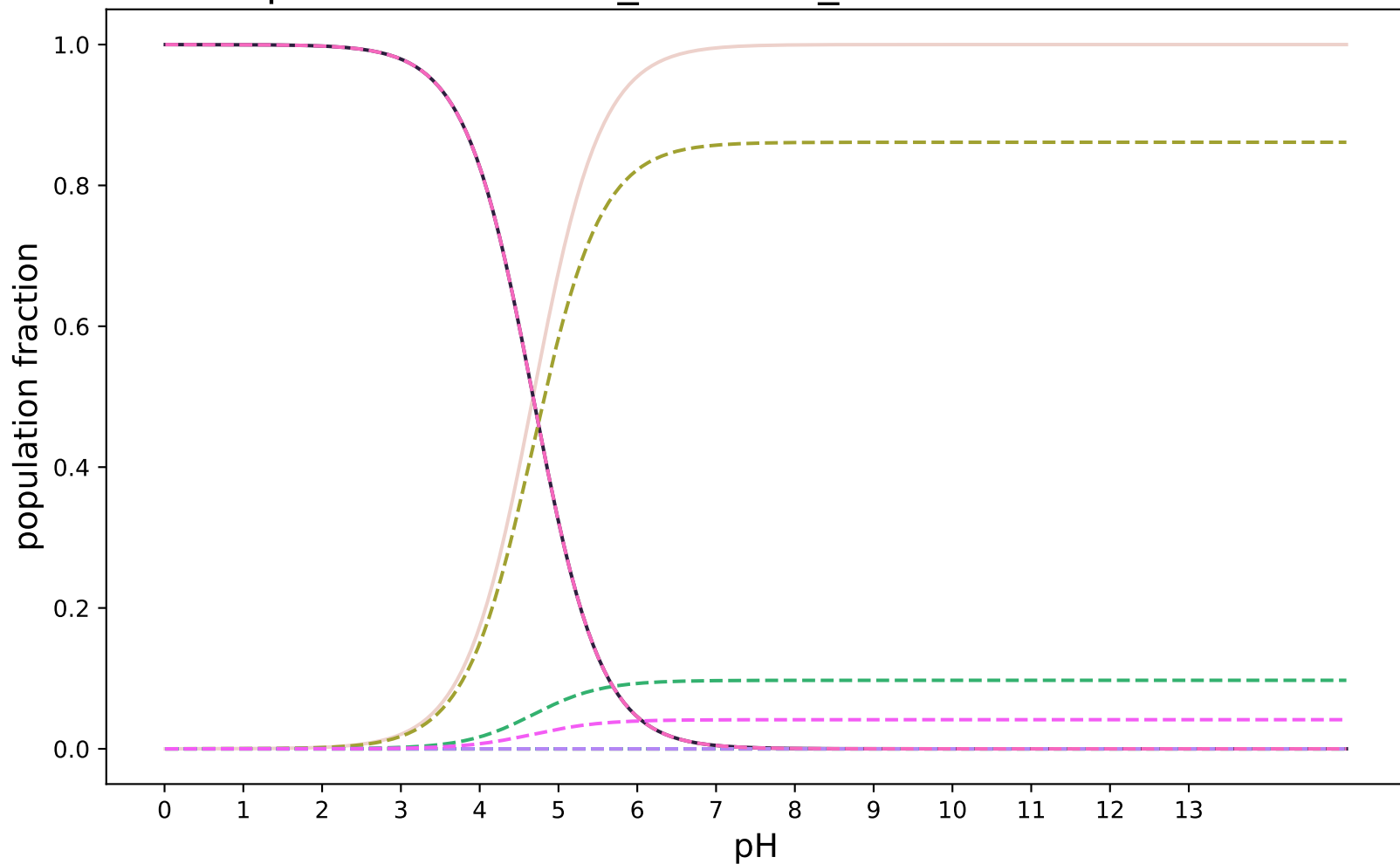
pKa-RobertRaddi_XGBoost_modified:SAMPL8-3
