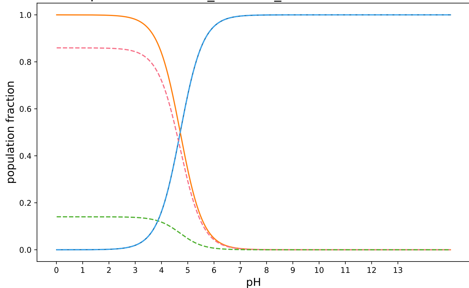
pKa-RobertRaddi_XGBoost_modified:SAMPL8-8
