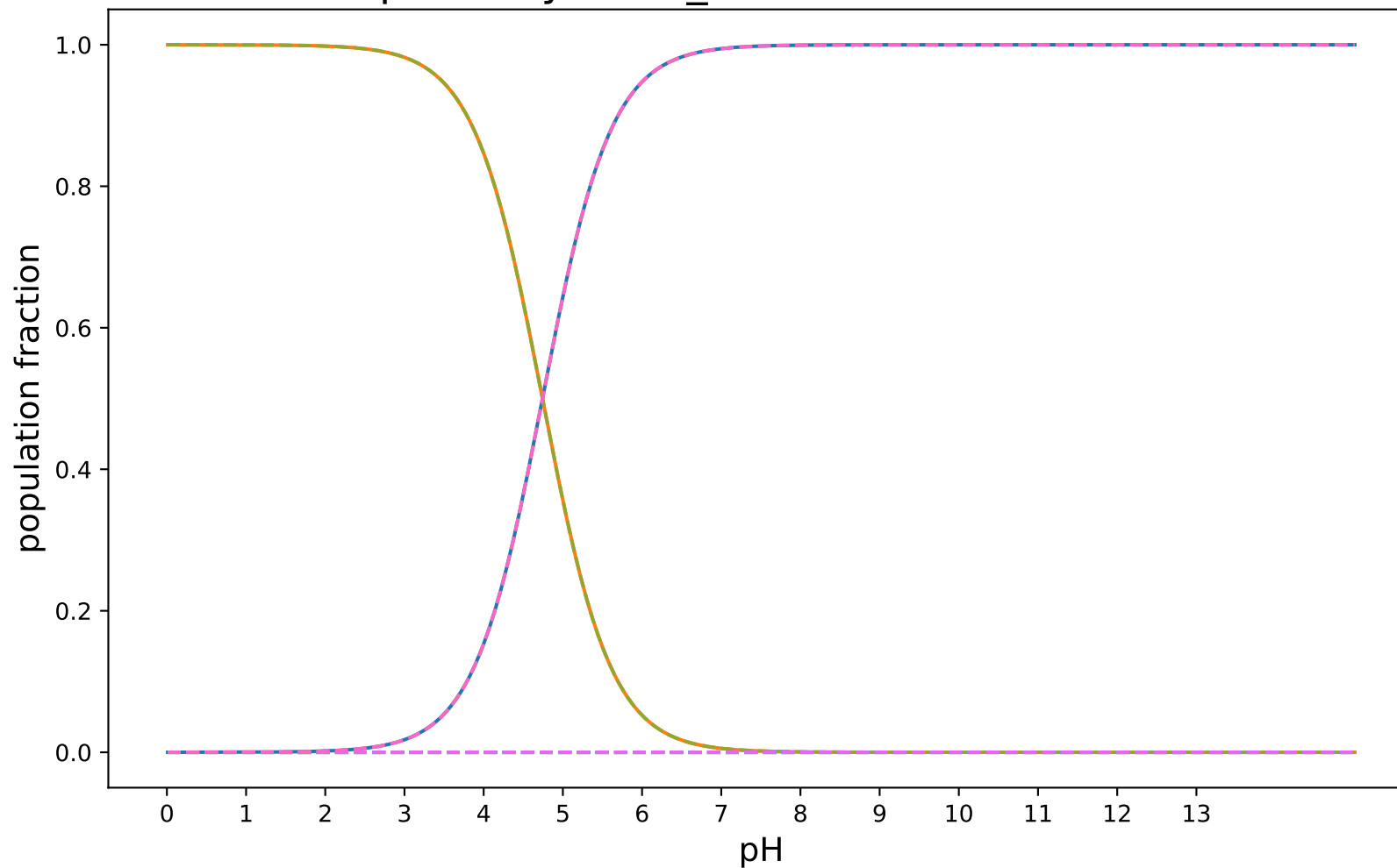
pKa-ZhiyiWu-1_modified:SAMPL8-16
