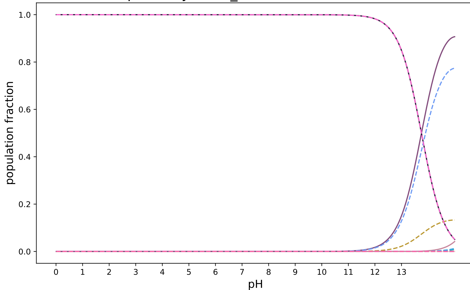
pKa-ZhiyiWu-1_modified:SAMPL8-21
