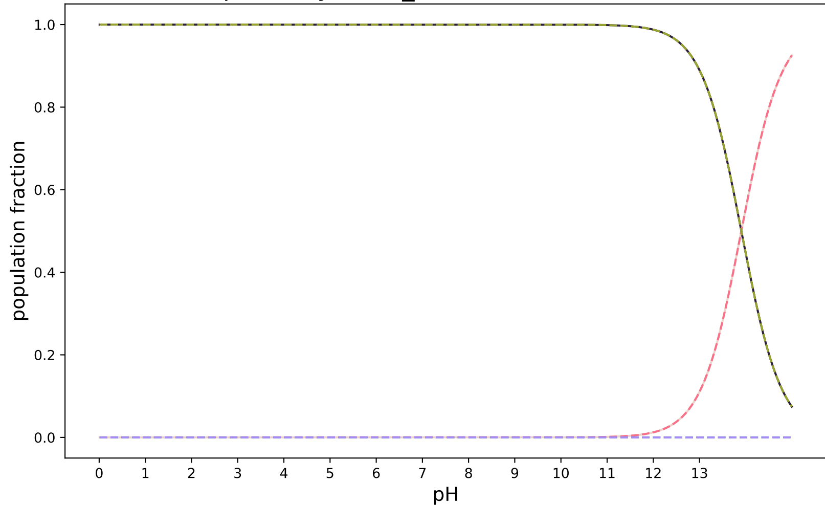
pKa-ZhiyiWu-1_modified:SAMPL8-22
