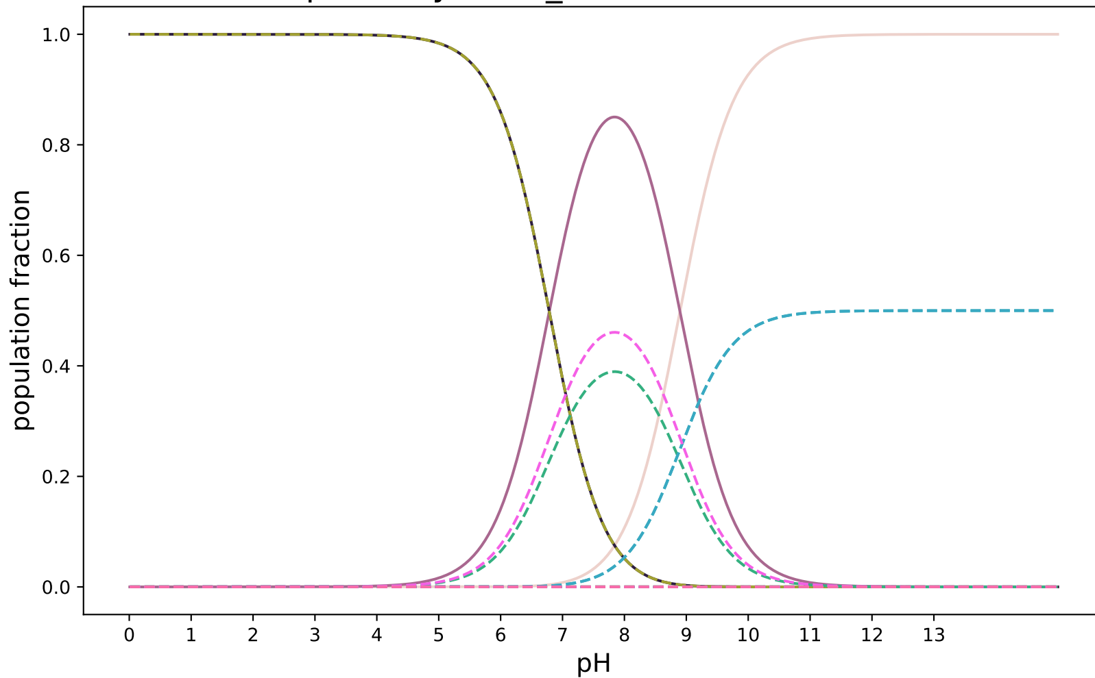
pKa-ZhiyiWu-1_modified:SAMPL8-3
