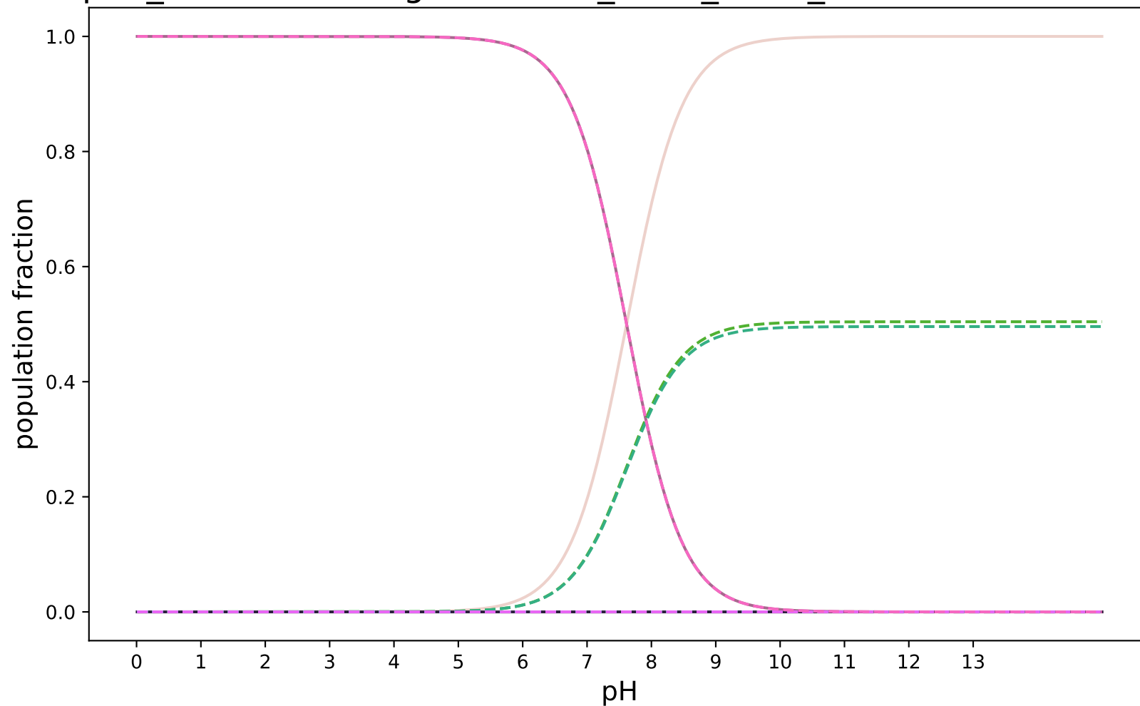
pKa_SabatinoRodriguezPaluch_uESE_extra_modified:SAMPL8-1
