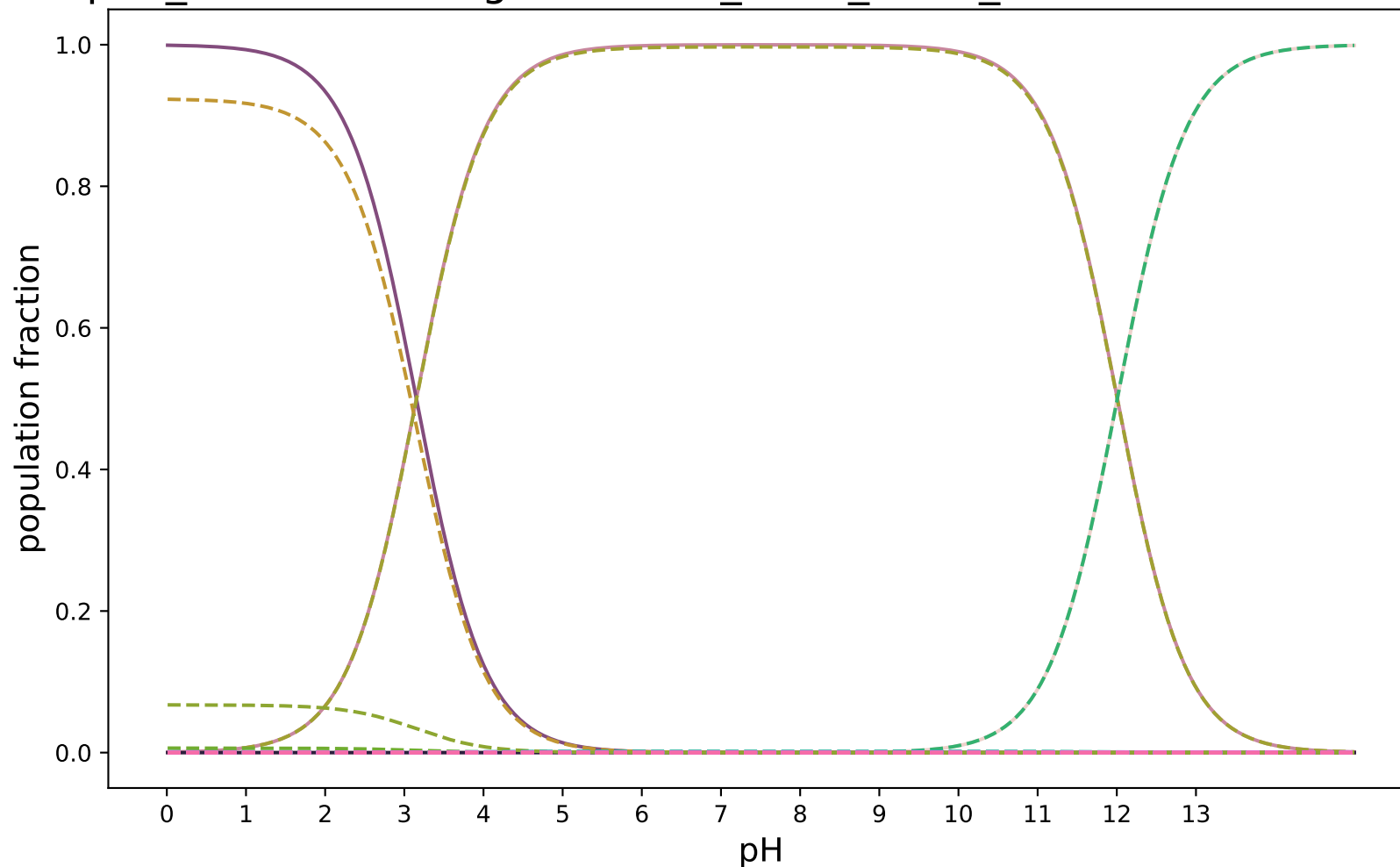
pKa_SabatinoRodriguezPaluch_uESE_extra_modified:SAMPL8-19
