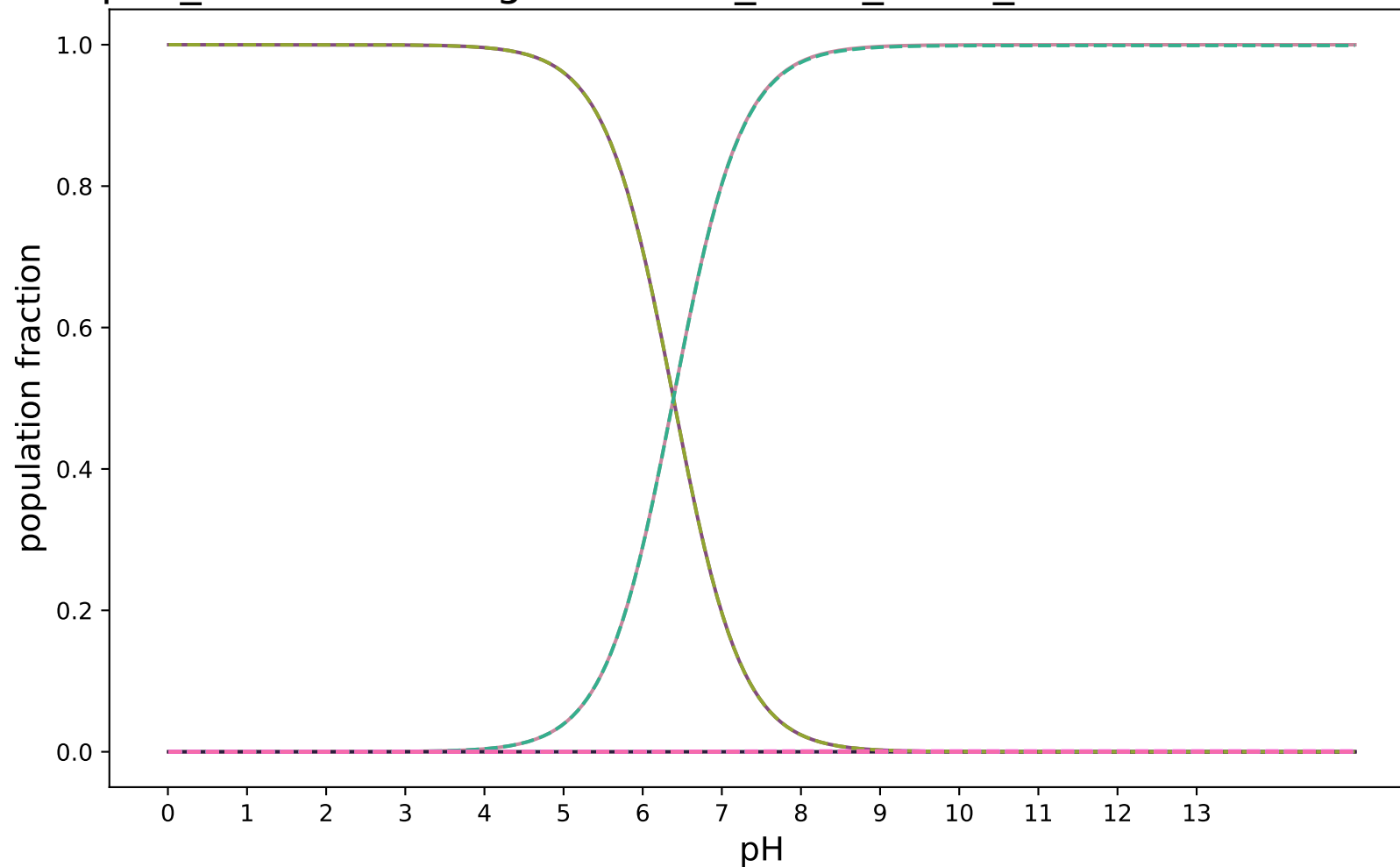
pKa_SabatinoRodriguezPaluch_uESE_extra_modified:SAMPL8-3
