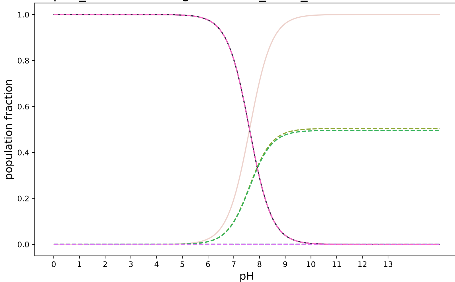
pKa_SabatinoRodriguezPaluch_uESE_modified:SAMPL8-1
