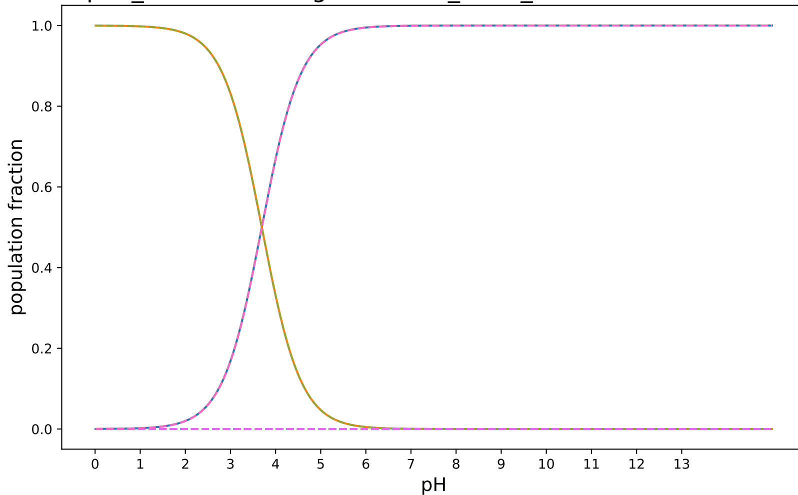
pKa_SabatinoRodriguezPaluch_uESE_modified:SAMPL8-16
