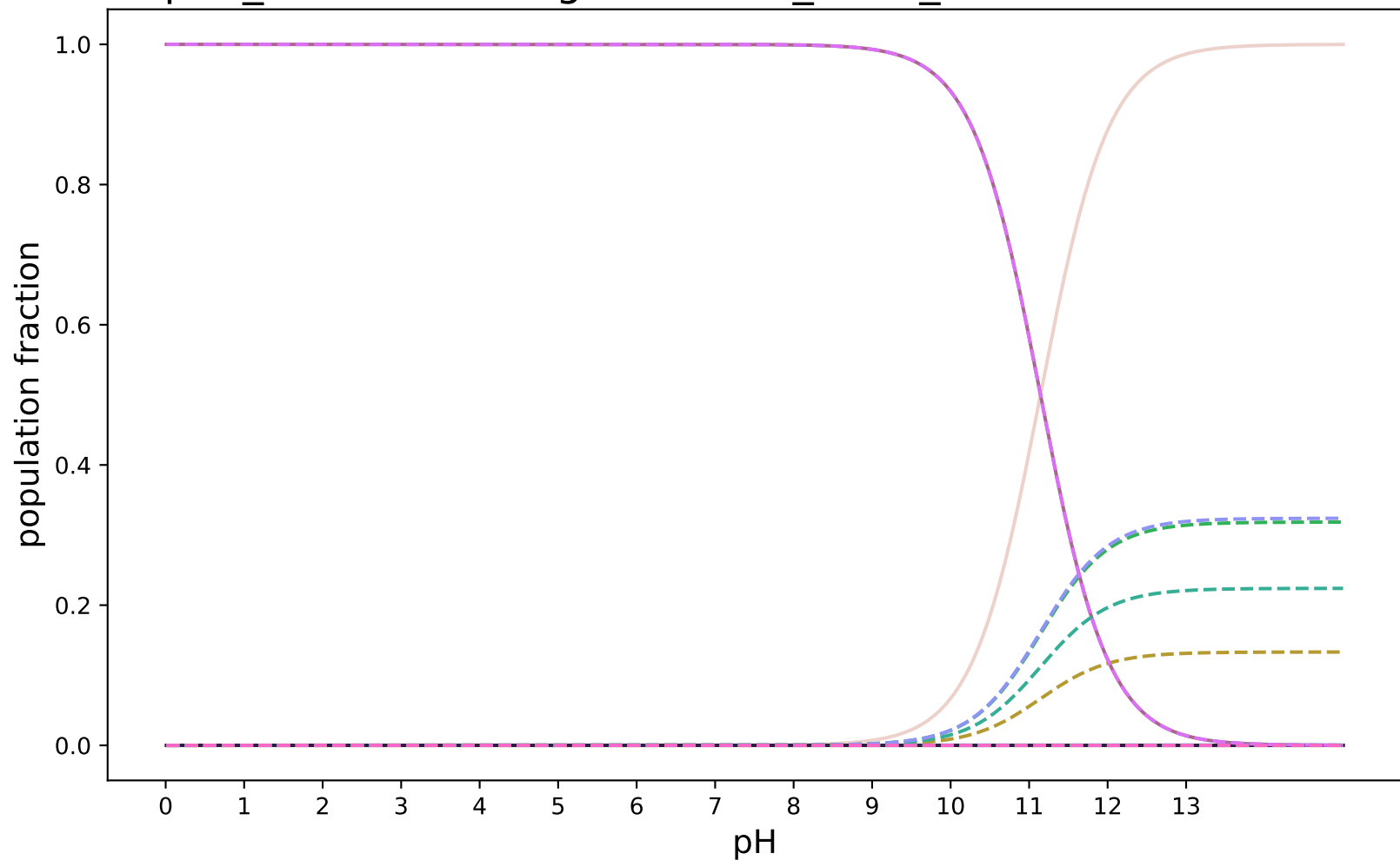
pKa_SabatinoRodriguezPaluch_uESE_modified:SAMPL8-4
