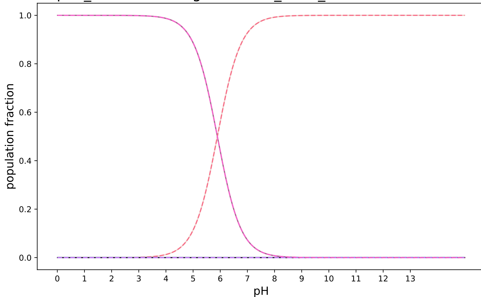
pKa_SabatinoRodriguezPaluch_uESE_modified:SAMPL8-6
