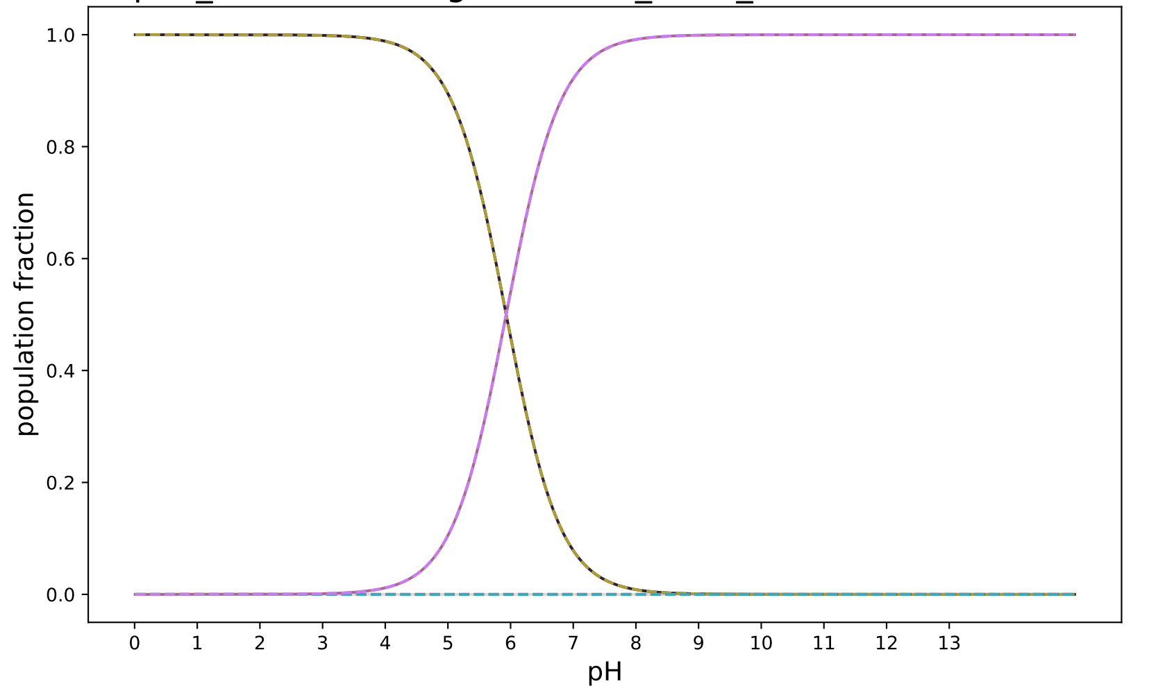
pKa_SabatinoRodriguezPaluch_uESE_modified:SAMPL8-9
