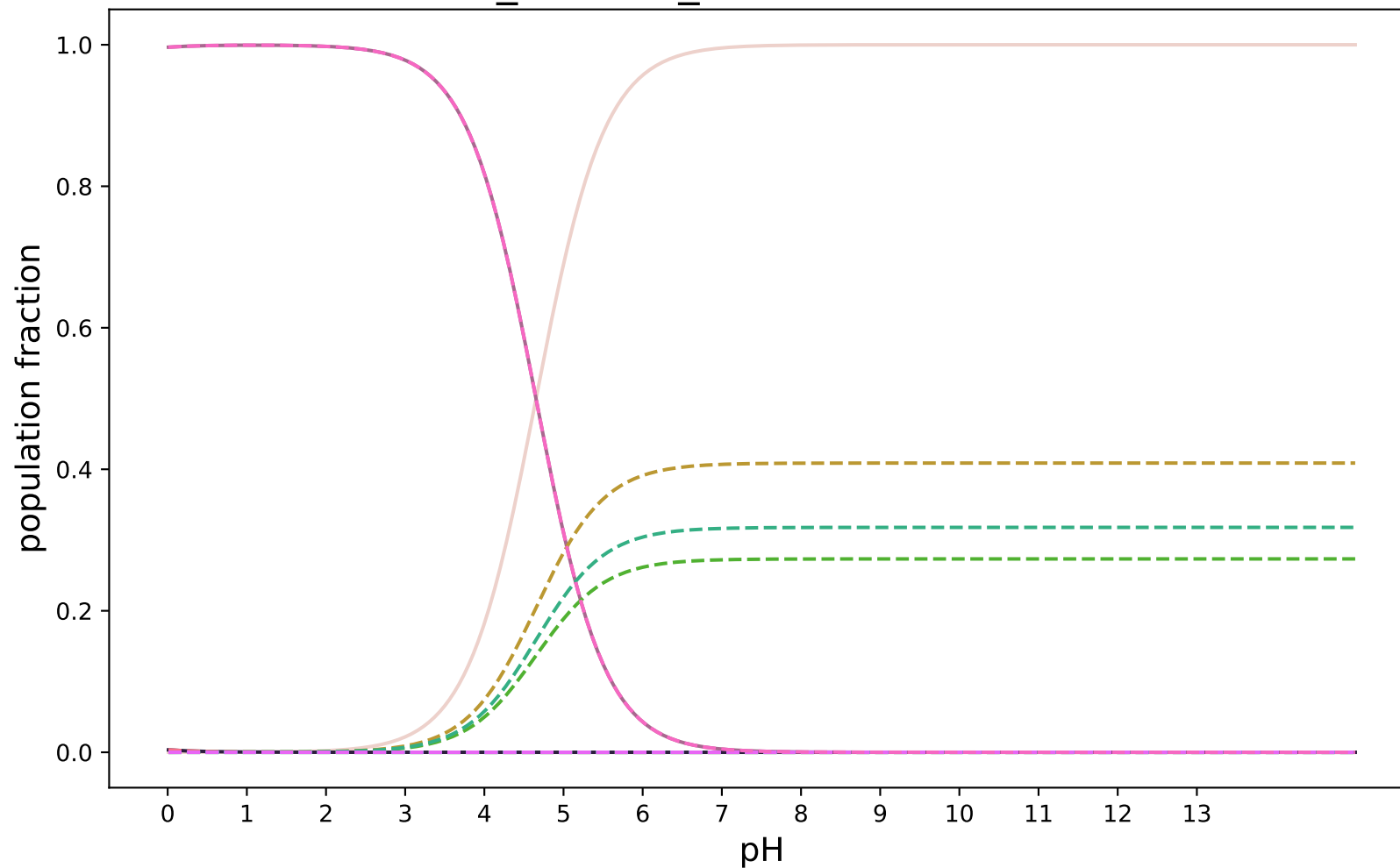
PKA_ECRISM_modified:SAMPL8-1
