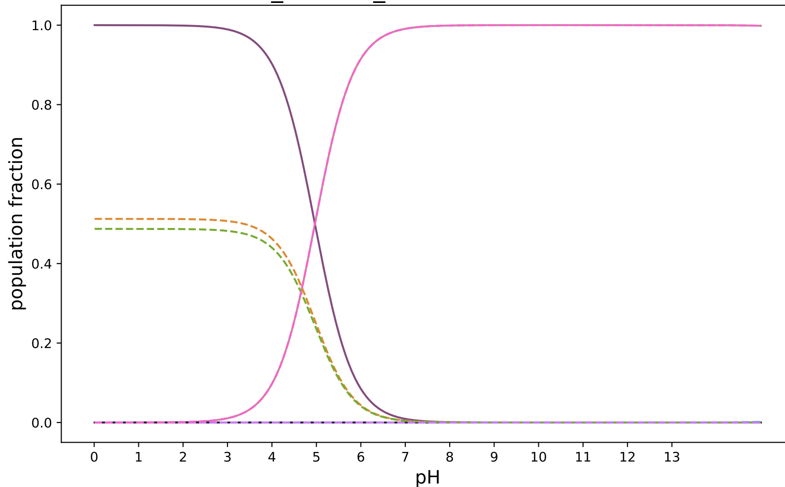
PKA_ECRISM_modified:SAMPL8-12
