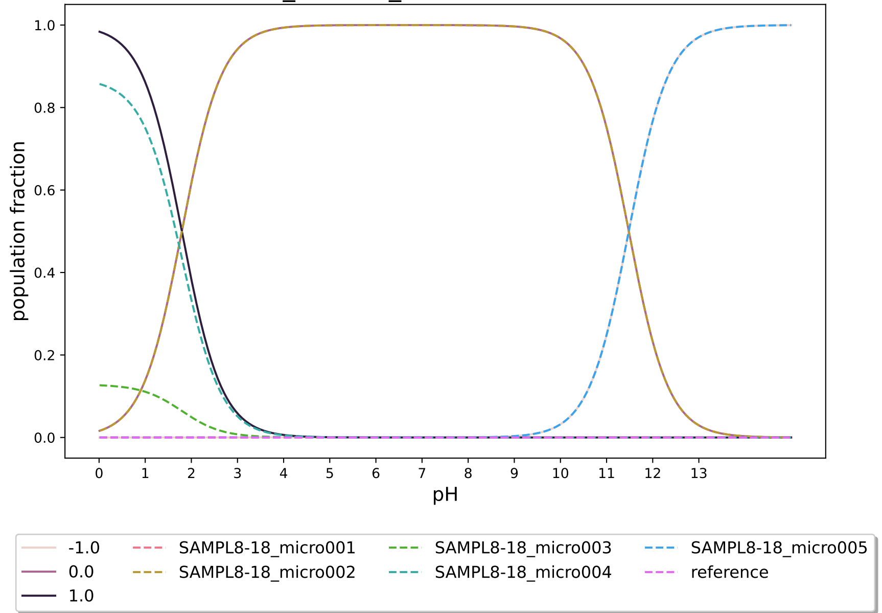
PKA_ECRISM_modified:SAMPL8-18
