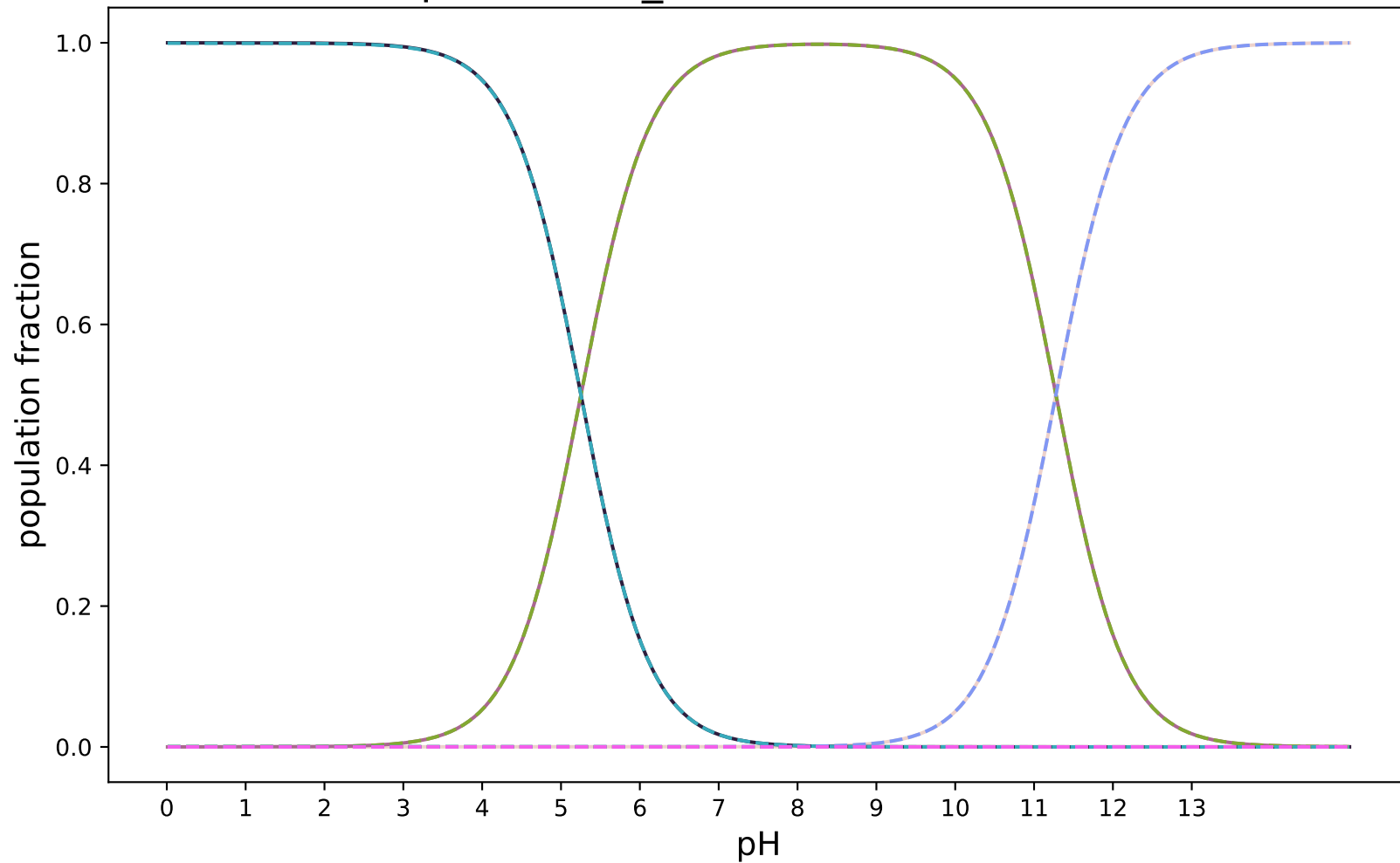
pKa-3DS-1_modified:SAMPL8-18
