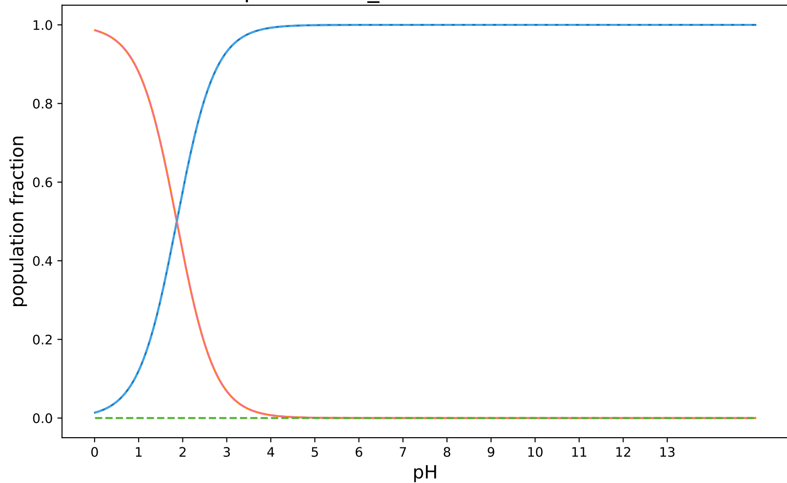
pKa-3DS-1_modified:SAMPL8-8
