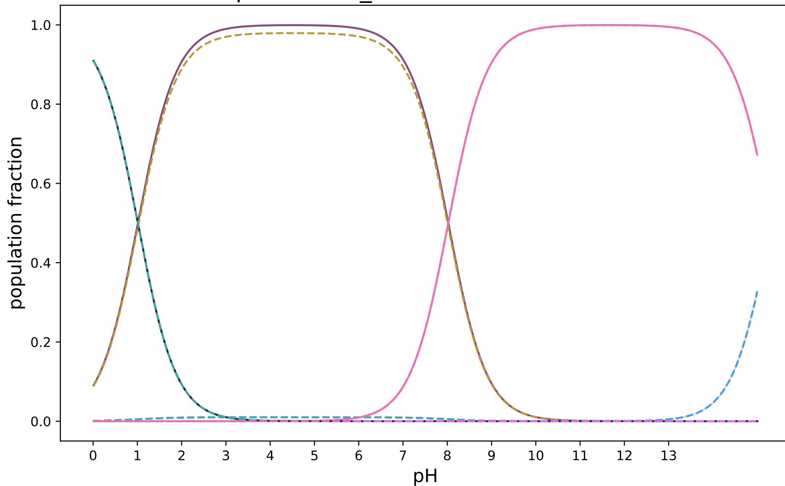
pKa-3DS-2_modified:SAMPL8-12
