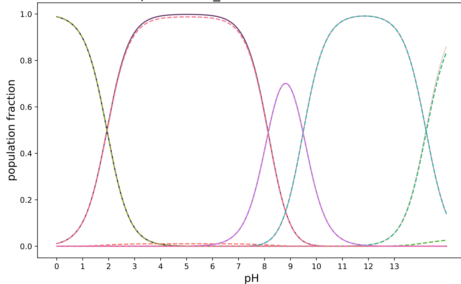
pKa-3DS-2_modified:SAMPL8-14
