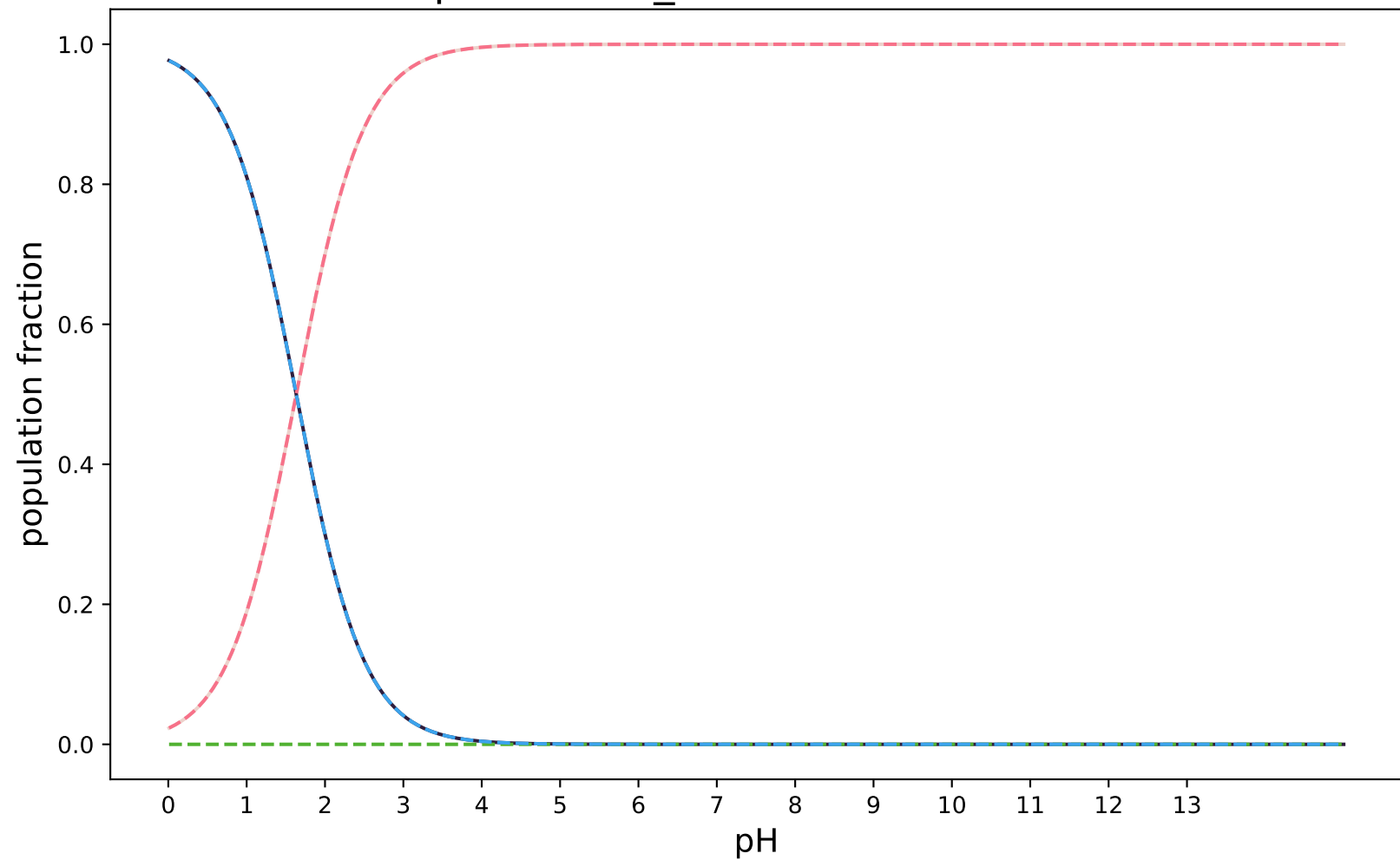
pKa-3DS-2_modified:SAMPL8-2
