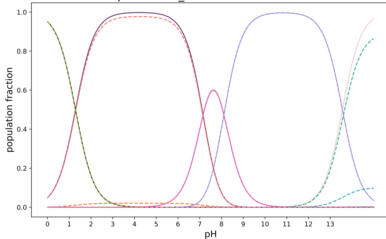
pKa-3DS-2_modified:SAMPL8-21
