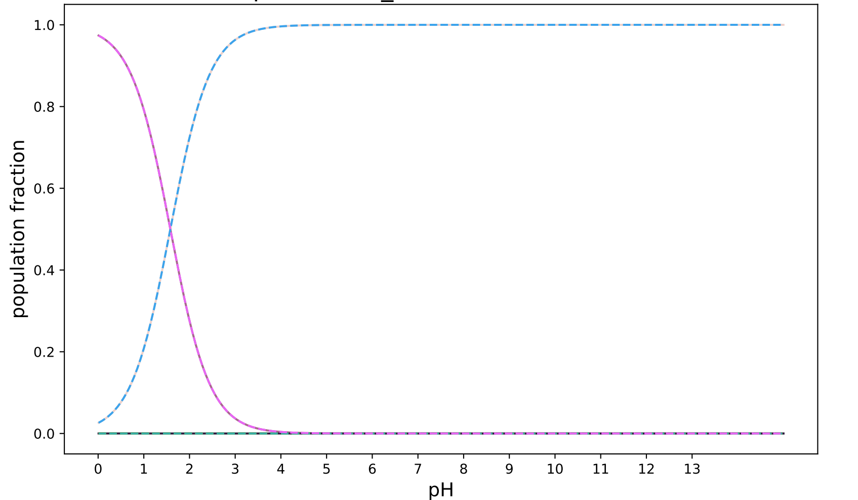
pKa-3DS-2_modified:SAMPL8-5
