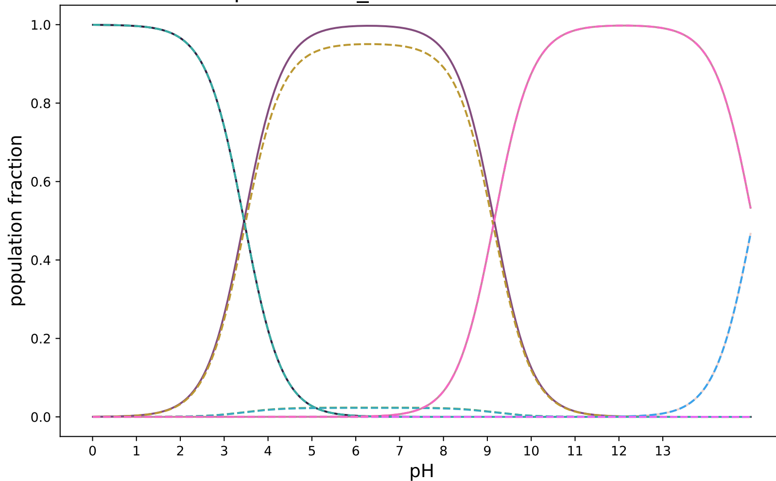
pKa-3DS-3_modified:SAMPL8-12
