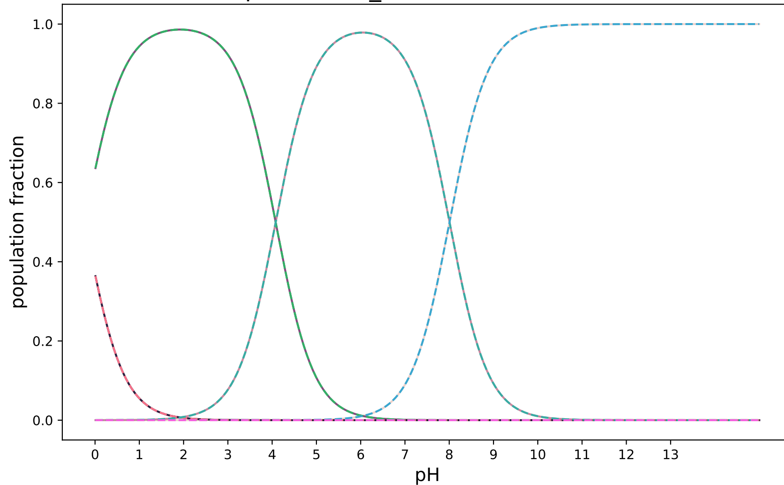
pKa-3DS-3_modified:SAMPL8-3
