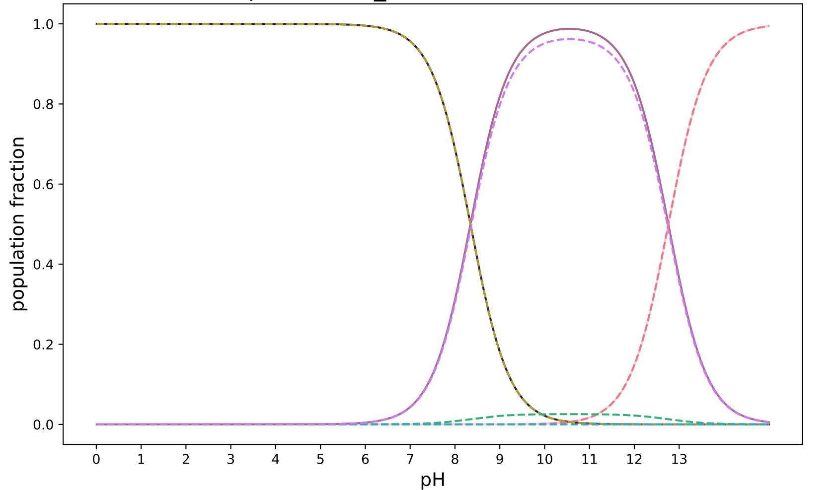
pKa-3DS-3_modified:SAMPL8-9
