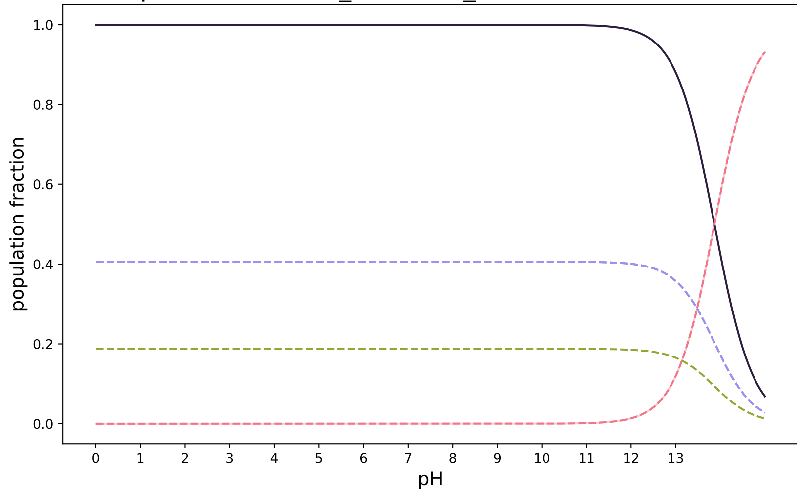
pKa-RobertRaddi_AdaBoost_modified:SAMPL8-12
