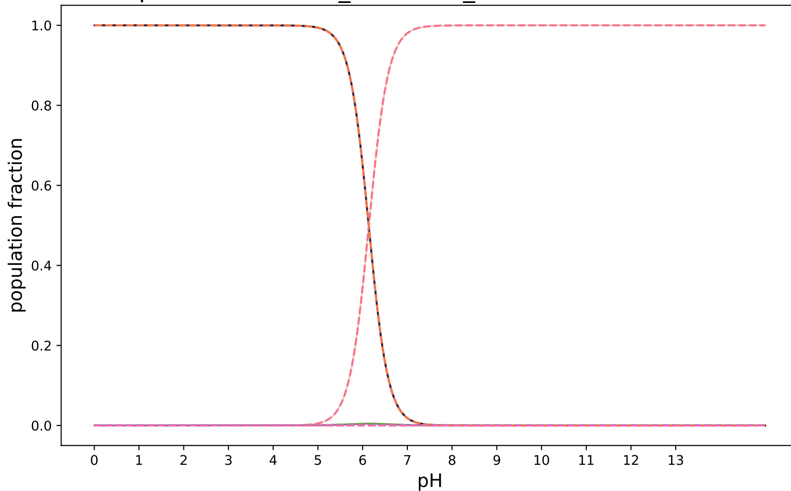
pKa-RobertRaddi_AdaBoost_modified:SAMPL8-14
