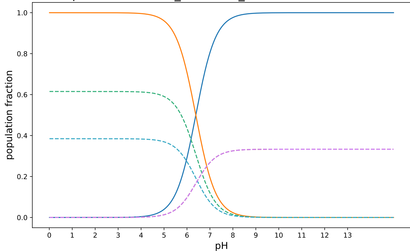
pKa-RobertRaddi_AdaBoost_modified:SAMPL8-15
