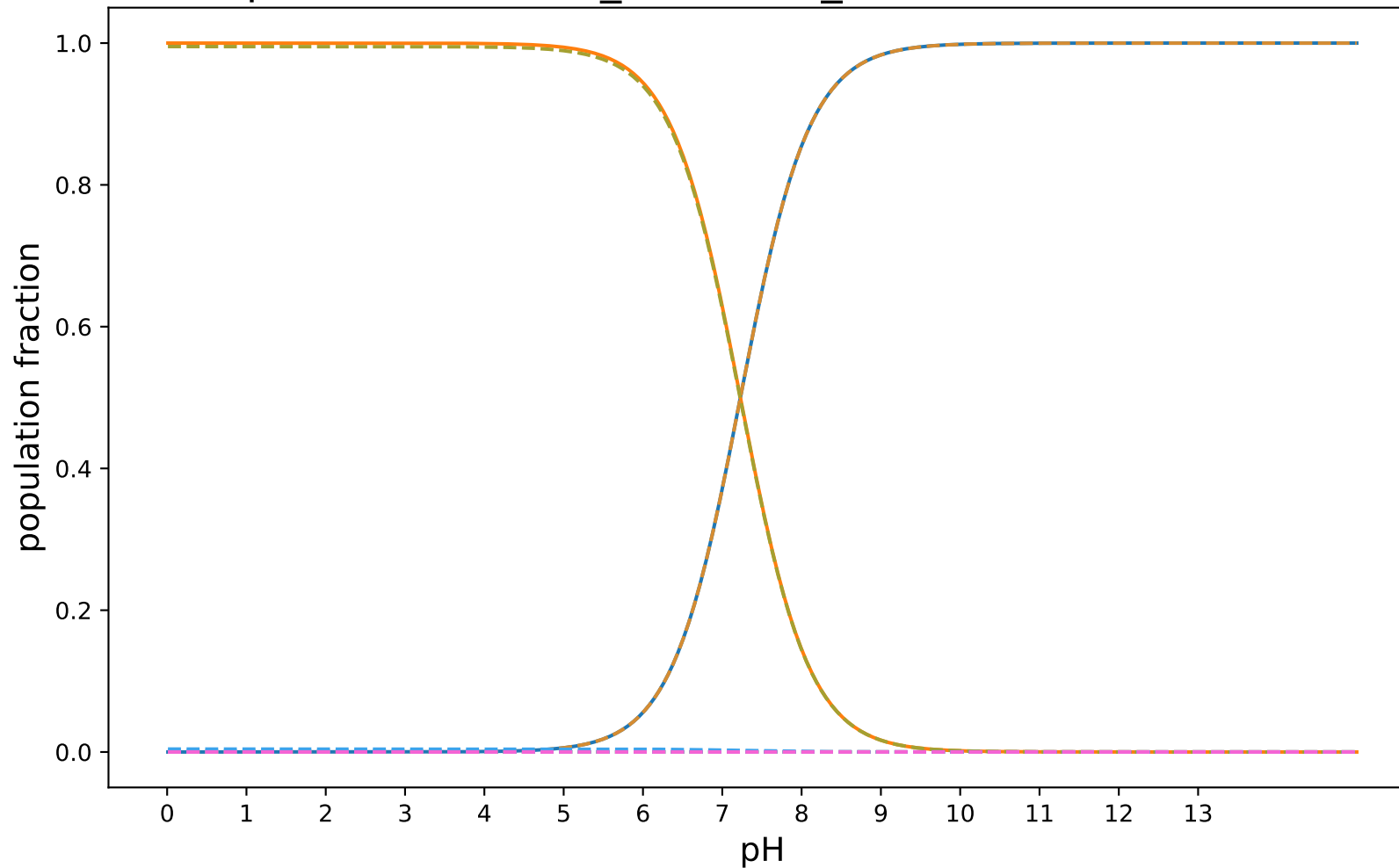
pKa-RobertRaddi_AdaBoost_modified:SAMPL8-16
